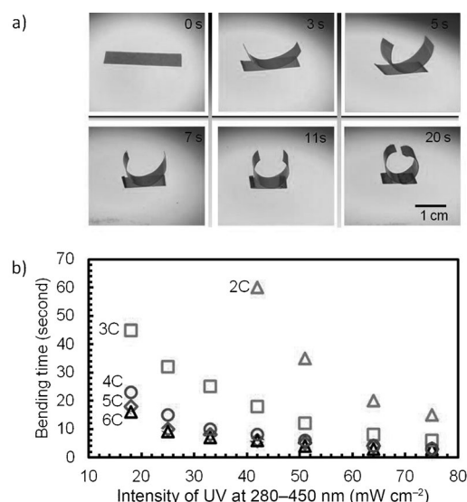
Figure 2. a) A series of photographs demonstrating the macroscopic photoinduced bending of a poly2C film (25 mm × 10 mm × 0.2 mm) by UV-light irradiation at \lambda = 280–450 nm. The final shape remained stable after the light was turned off. b) Bending time versus UV-light intensity in various polymers with different methylene groups in the corresponding glycols. It showed different bending speeds under the same conditions of UV-light irradiation, with the speed clearly increasing with increased carbon chain length from 2C to 4C and keeping a similar speed as 4C, 5C, and 6C. Legends such as 2C, 3C, 4C, 5C, and 6C refer to poly2C, poly3C, poly4C, poly5C, and poly6C, respectively.
